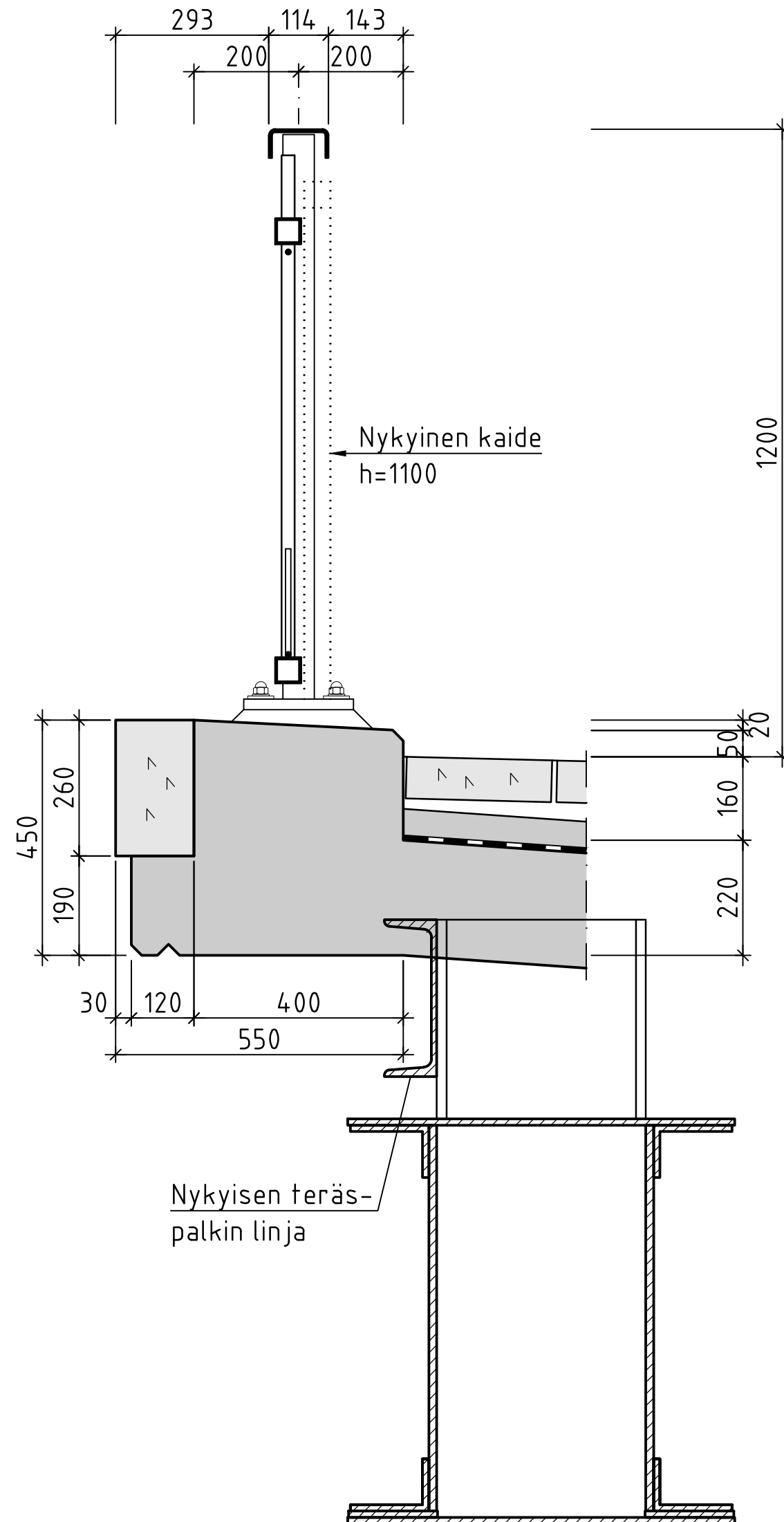
KAIDE, 1:10
